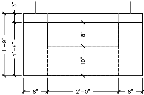
TOP SLAB PLAN VIEW
