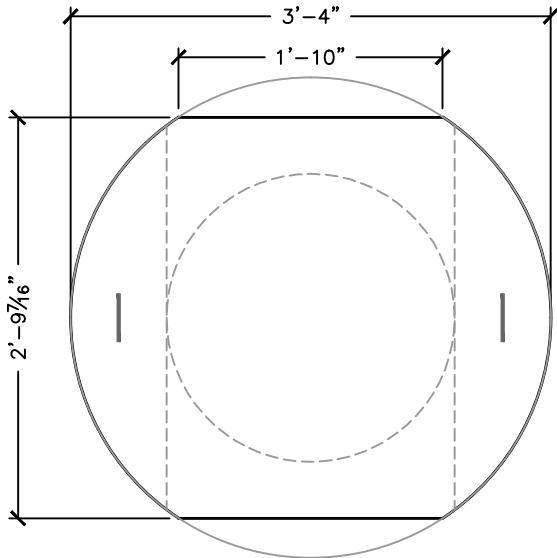
TOP SLAB PLAN VIEW
